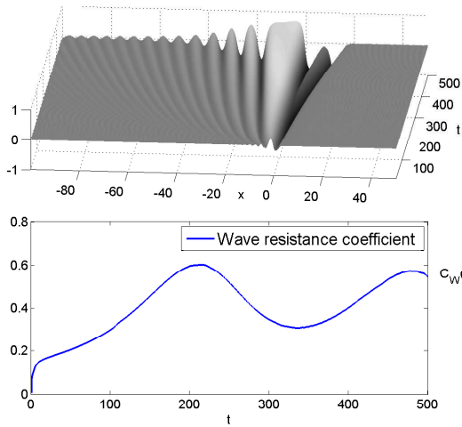
(a) \delta = 5/12 .
