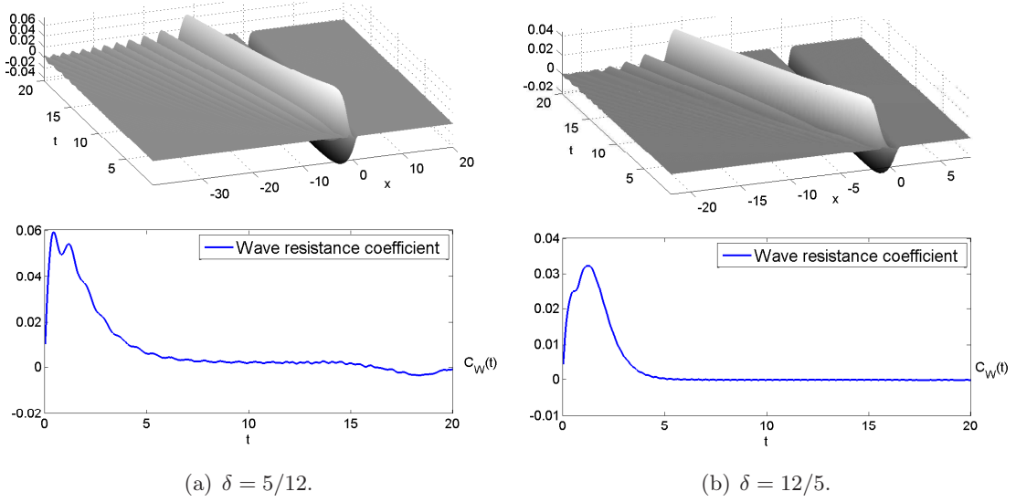
FIGURE 7. Supercritical flow: \text{Fr} = 1.5 . \alpha = \epsilon_2 = \mu = 0.1 , \gamma = 0.99 .
