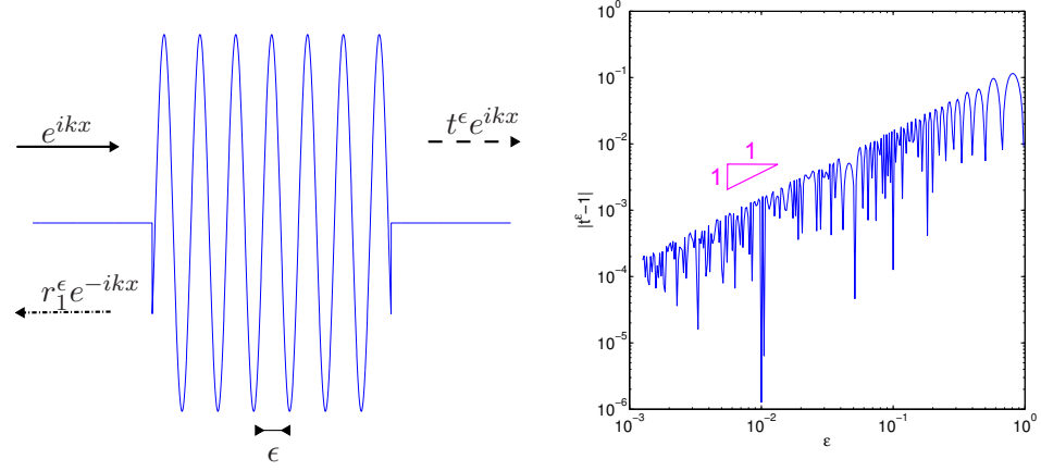
(a) \theta = 0 .
