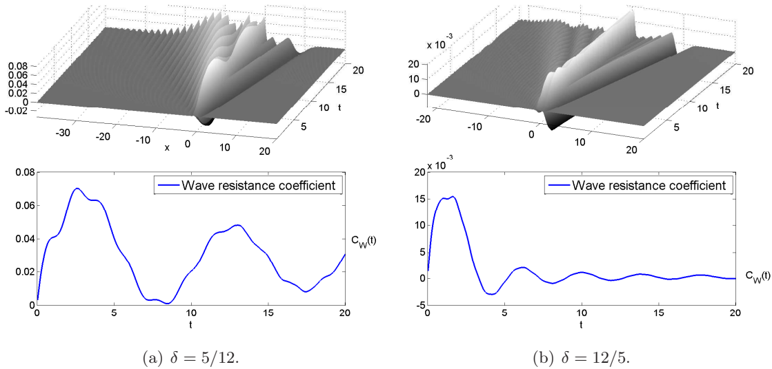
FIGURE 6. Subcritical flow: \text{Fr} = 0.5 . \alpha = \epsilon_2 = \mu = 0.1 , \gamma = 0.99 .
