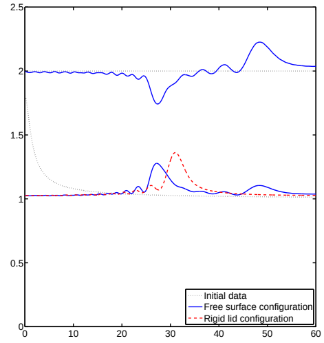
(b) t = 40 . \epsilon = 0.1, \delta = 1, \gamma = 1/4 .
