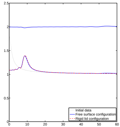
(b) t = 40 . \epsilon = 0.1, \delta = 1, \gamma = 9/10 .
