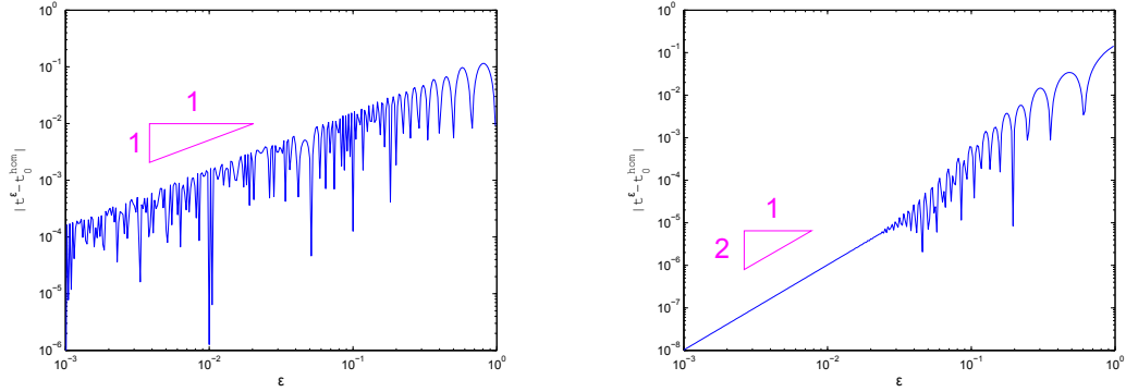
FIGURE 3. Plot of \log |t^\epsilon - t_0^{\text{hom}}| versus \log \epsilon^{-1} for the case of the potentials V_1^\epsilon(x; \theta) in (2.22) (left panel, slope 1), and V_2^\epsilon(x; \theta) in (2.23) (right panel, slope 2). One has k = 1 , and \theta = 0 .
