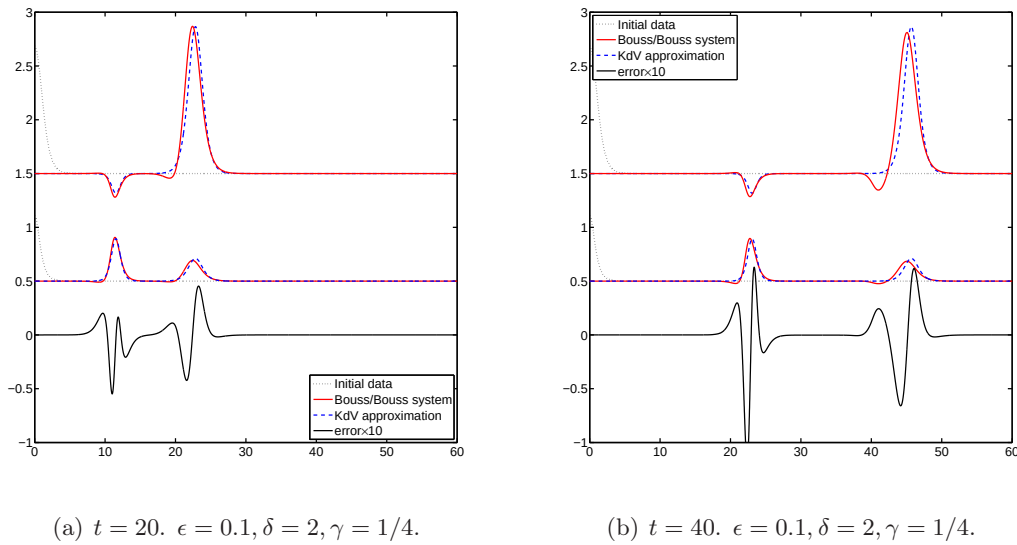
FIGURE 10. Solitary wave solution of the KdV approximation, and symmetric Boussinesq/Boussinesq model, at times (a) t=20 , (b) t=40 .
