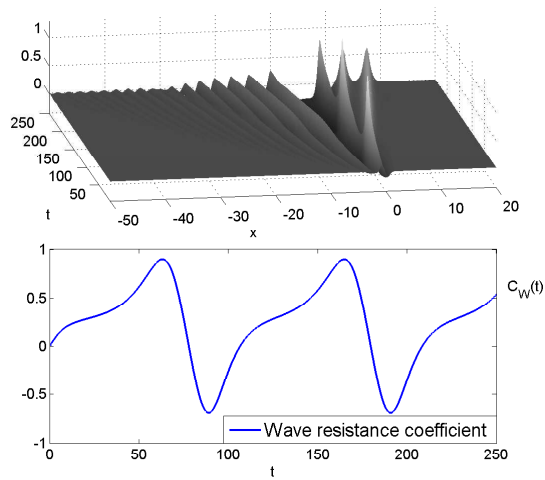
(b) \delta = 12/5 .
